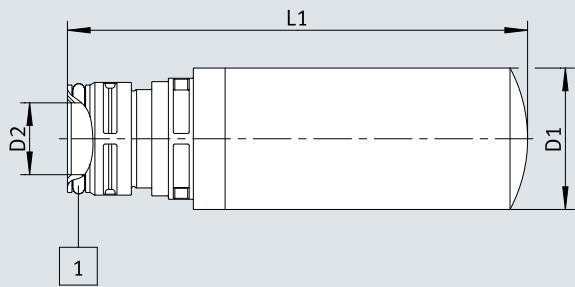
Dimensions – AMTX (long design)
