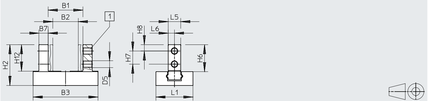
[1] Threaded hole for mounting the gripper fingers
