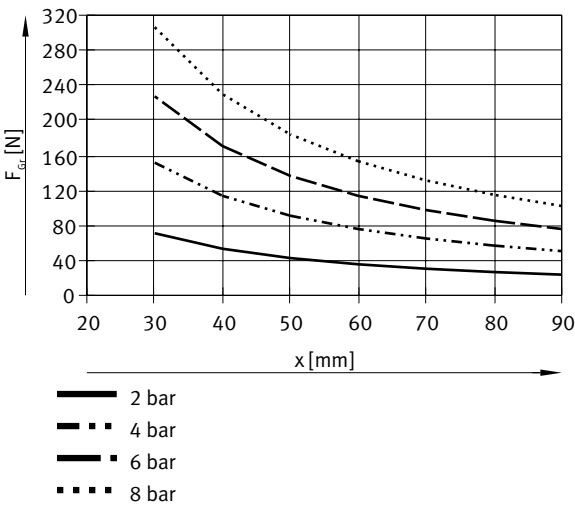
Gripping force F per gripper jaw as a function of operating pressure and lever arm x – Internal gripping (opening), double-acting – DHRC-32-A
