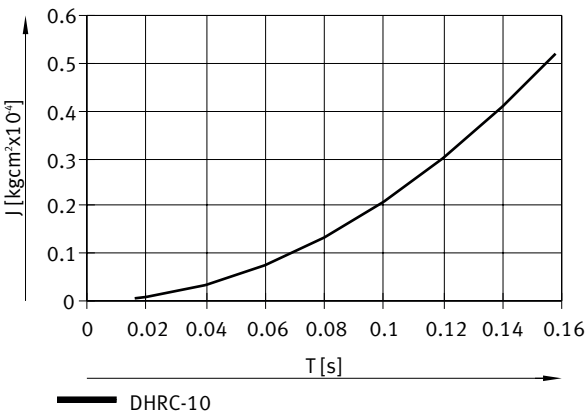
Opening and closing times T to be set at 0.6 MPa (6 bar, 87 psi) as a function of mass moment of inertia of the gripper fingers – DHRC-10
