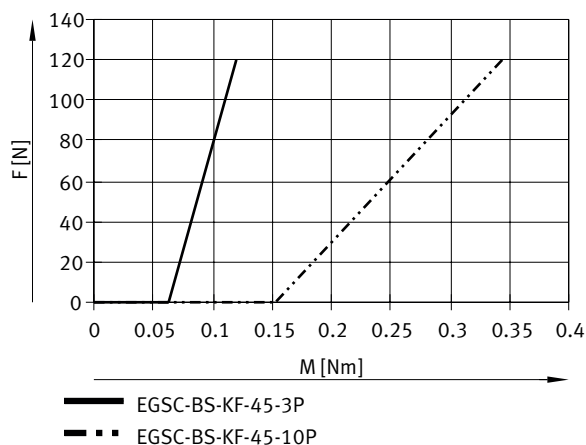
Feed force F as a function of input torque M for size 45
