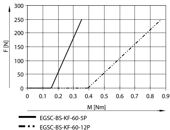
Feed force F as a function of input torque M for size 60
