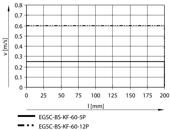
Speed v as a function of stroke l for size 60
