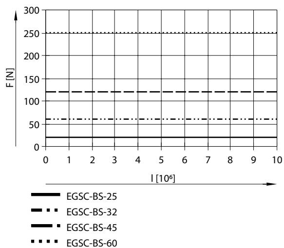
Feed force F as a function of service life l
