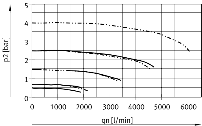
Standard flow rate q_n as a function of output pressure p_2 ( p_1 = 10 bar) MS6-LRP-3/8-D4/D5MS6-LRP-1/2-D4/D5
