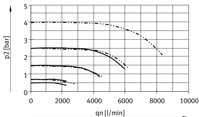
Standard flow rate q_n as a function of output pressure p_2 ( p_1 = 10 bar) MS6-LRP-3/8-D4/D5MS6-LRP-1/2-D4/D5
