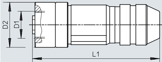
Dimensions – Socket NECU-M-B12G5, M12x1, 5-pin, straight
