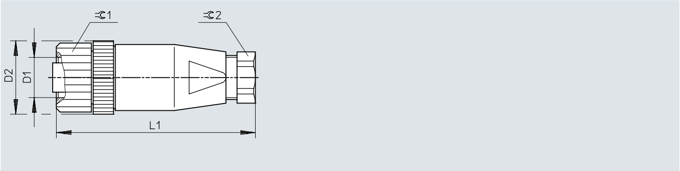
Dimensions – Socket SIE-GD, M12x1, 4-pin
