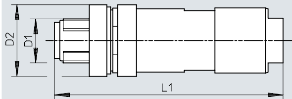
Dimensions – Plug NECU-M-S-A12G4-IS
