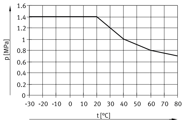
Operating pressure p as a function of temperature t (PLN)
