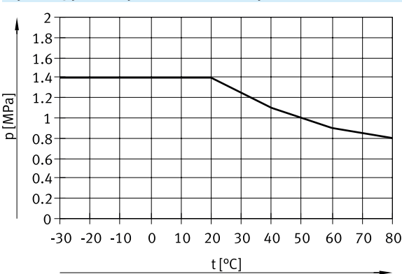
Operating pressure p as a function of temperature t (PAN-R; external Ø 22 ... 28 mm)
