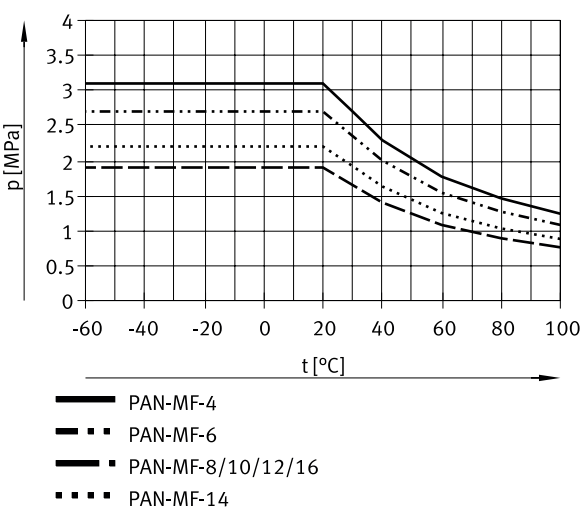
Operating pressure p as a function of temperature t (PAN-MF)
