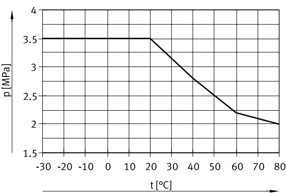
Operating pressure p as a function of temperature t (PAN-R; external Ø 4 ... 16 mm)
