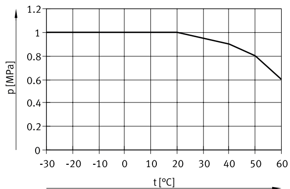
Operating pressure p as a function of temperature t (PEN)
