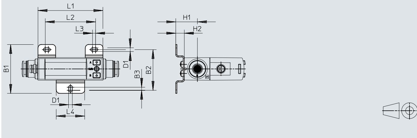
Dimensions – Wall mounting SAMH-FH-W
