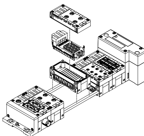
Modularity with electrical peripherals CPX
