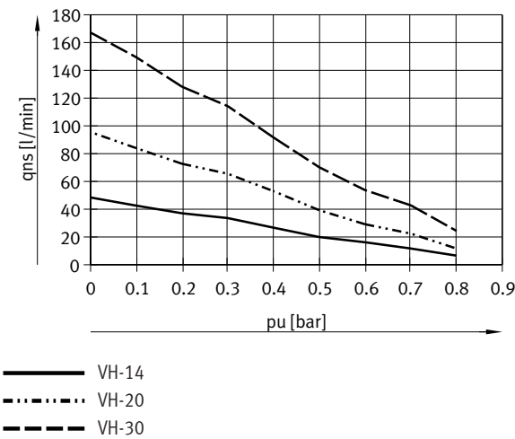
Pressure ratios, suction rate q_{ns} as a function of negative pressure p_u , p_1 and operating pressure 6 bar VH-1 4/20/30 VL-1 4/20
