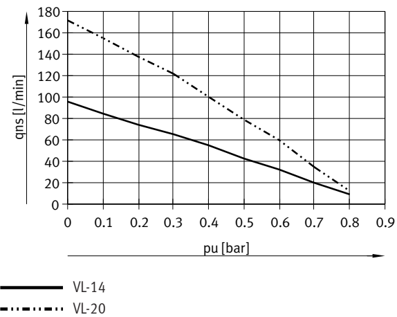
Pressure ratios, suction rate q_{ns} as a function of negative pressure p_u , p_1 and operating pressure 6 bar VH-1 4/20/30 VL-1 4/20
