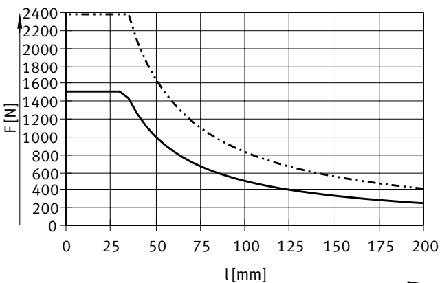
DFM-80 ... 100-GF, 行程 25 mm
