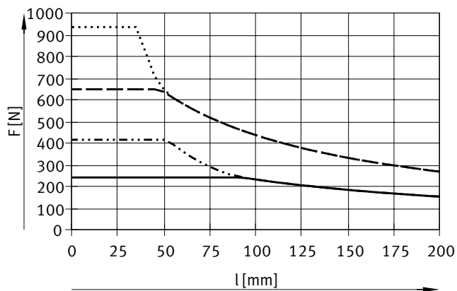
DFM-32 ... 63-KF, 行程 125 ... 200 mm
