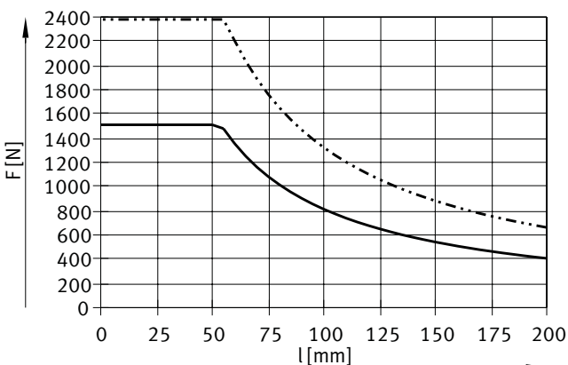
DFM-80 ... 100-GF, 行程 80 ... 200 mm
