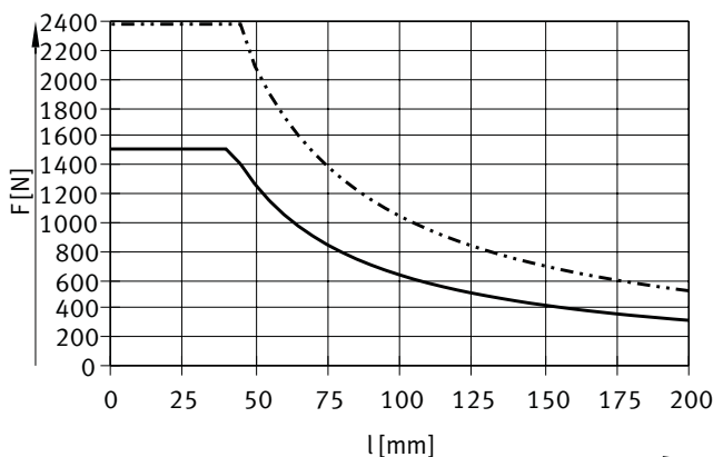
DFM-80 ... 100-GF, 行程 50 mm
