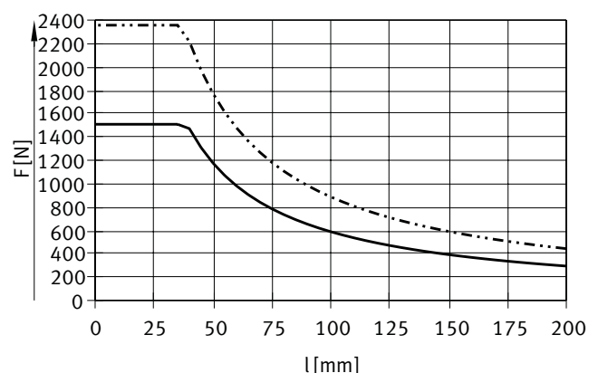
DFM-80 ... 100-KF, 行程 80 ... 200 mm
