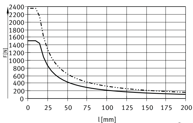
DFM-80 ... 100-KF, 行程 50 mm
