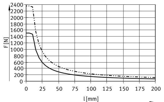
DFM-80 ... 100-KF, 行程 25 mm
