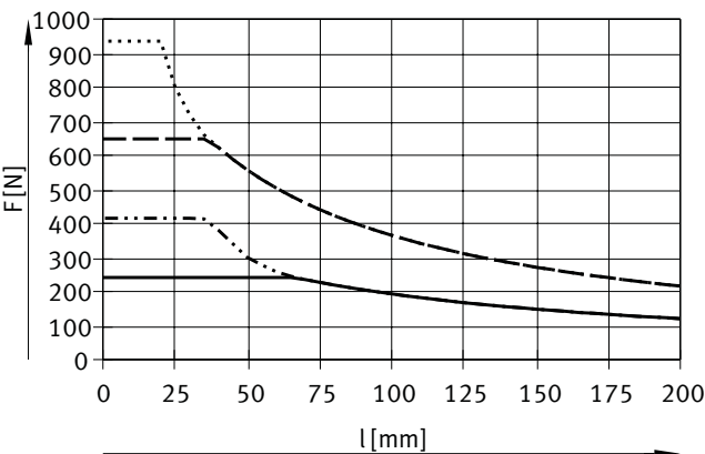
DFM-32 ... 63-KF, 行程 80 ... 100 mm
