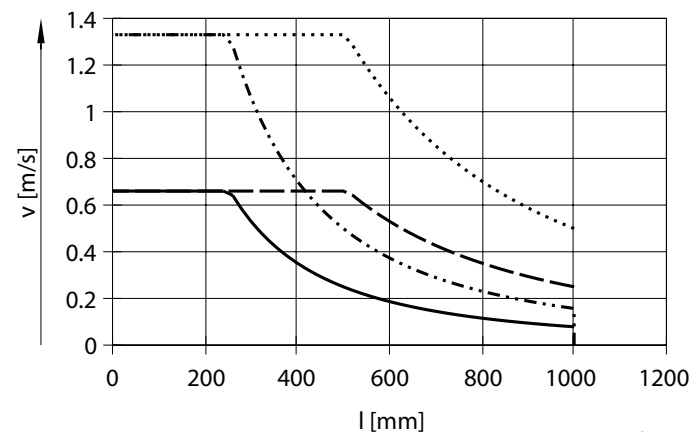
— ELGD-100-5P - - - ELGD-100-10P - - - ELGD-100-5P-SU ..... ELGD-100-10P-SU
