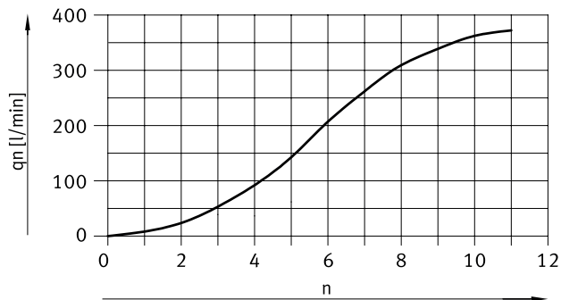
Standard nominal flow rate q_n at 6 → 5 bar as a function of spindle rotations n (GRO-1/4)
