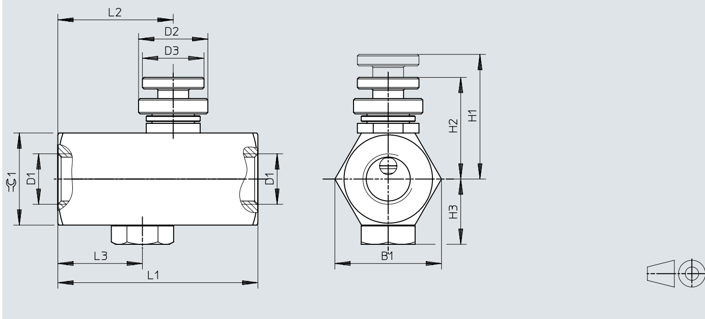
Dimensions – GRO-1/4
