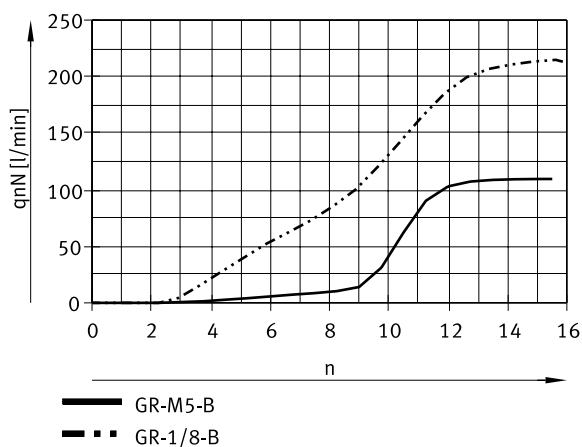
Standard nominal flow rate q_{pN} at 6 → 5 bar as a function of spindle rotations n (GRO-M5-B, GRO-1/8-B)
