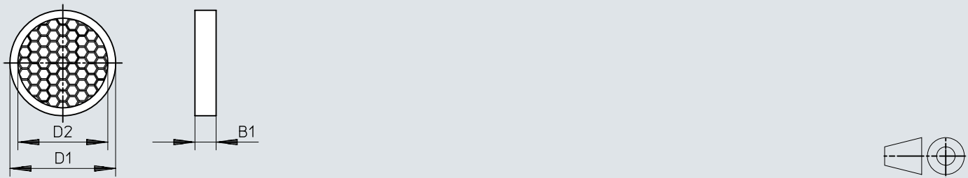
Dimensions – Reflector SARA-R-D20-M
