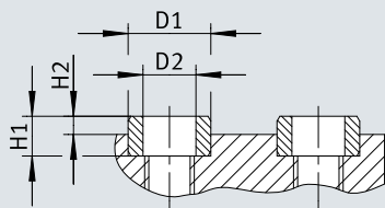
Dimensions – Parallel gripper HEAC with centring sleeve ZBH
